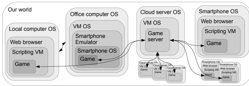
Figure 2: A partial, simplified visualization of locational dependencies in a hypothetical scenario of a development of a virtual reality game described in the text. OS is Operating System, VM is Virtual Machine, arrows indicate selected connections and interactions. This chart only shows programs related to a single instance of the game in each software environment; other (possibly identical) programs running simultaneously in each environment are not shown. For simplicity, advertisement software spanning across multiple devices and systems is also not shown. Cloud servers and smartphones may appear and disappear in time.
